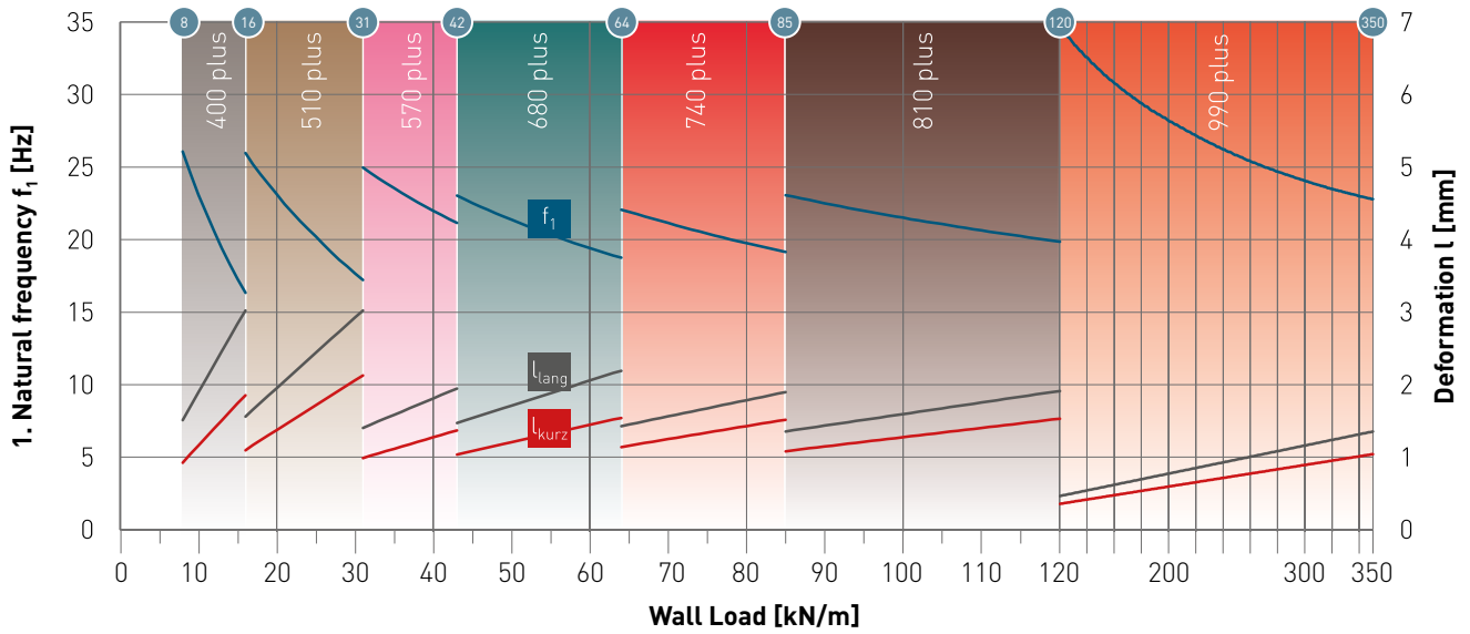
For wall width 140 mm
